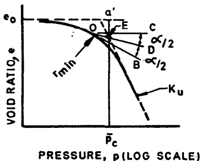
FIG. 14 GRAPHICAL CONSTRUCTION FOR DETERMINING FORMER MAXIMUM PRESSURE \bar{p}_c FROM e -LOG p CURVE
