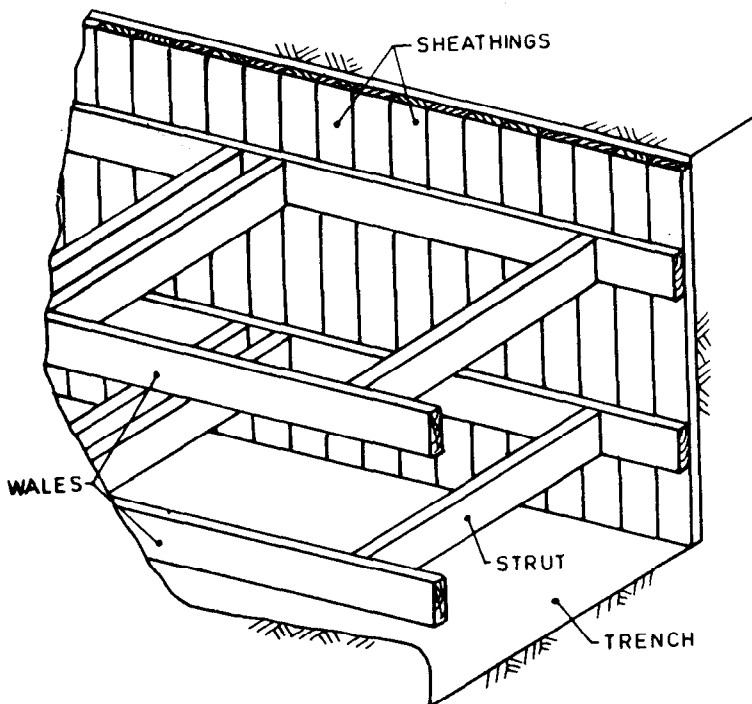
FIG. 1 ILLUSTRATIVE SKETCH SHOWING TIMBERING IN LOOSE SOIL
