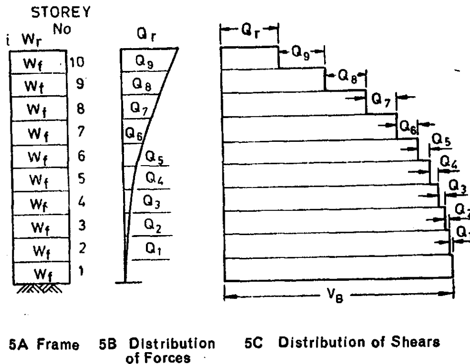
FIG. 5 FORCE AND SHEAR DISTRIBUTION FOR TEN-STOREYED BUILDING
