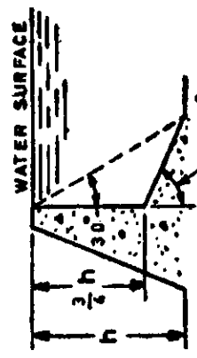
SHAPE B-4
