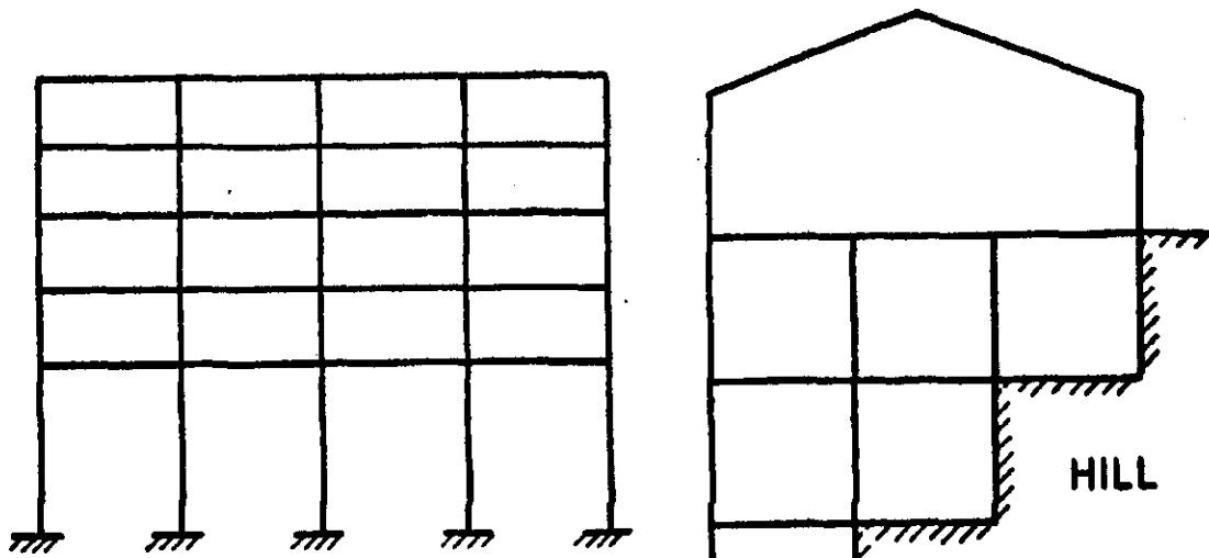
BUILDING WITH FLEXIBLE FIRST STOREY [INCLUDING BUILDINGS LIKE ASSEMBLY HALLS AND CINEMA THEATRES WHERE THE CENTRAL AUDITORIUM (IN ONE STOREY) COVERS UP TO THREE STOREYS OF THE SIDE FLANKS]
