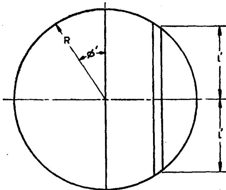
CIRCULAR TANK (PLAN)
