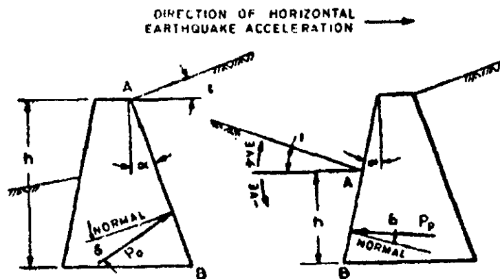
12A Active Pressure
