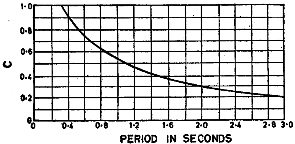
FIG. 3 C Versus PERIOD
