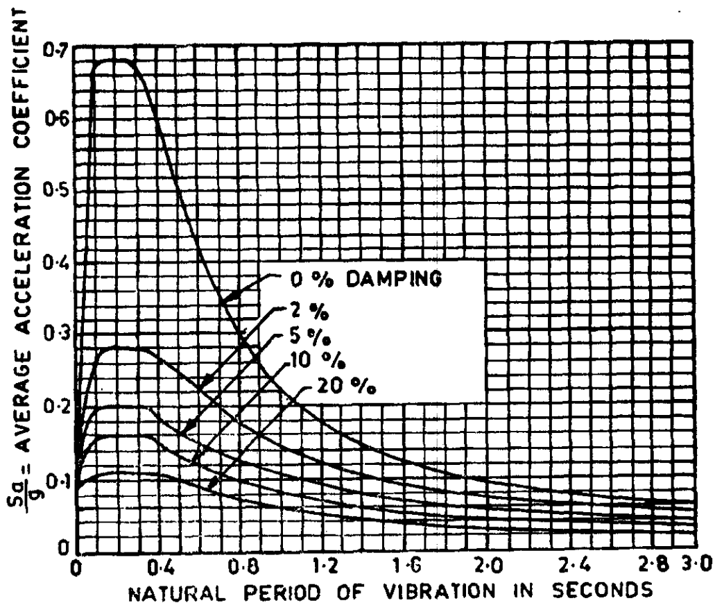
FIG. 2 AVERAGE ACCELERATION SPECTRA
