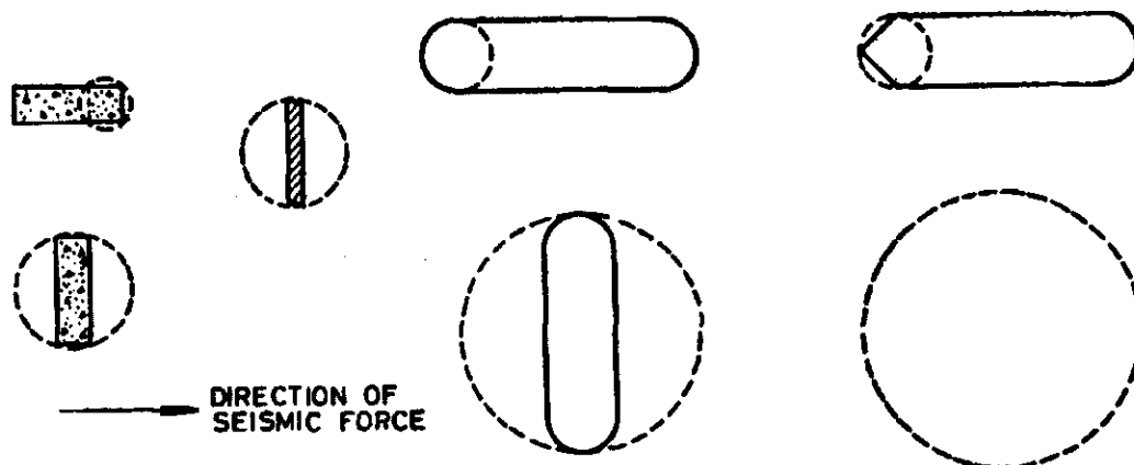
FIG. 9 CASES OF ENVELOPING CYLINDER
