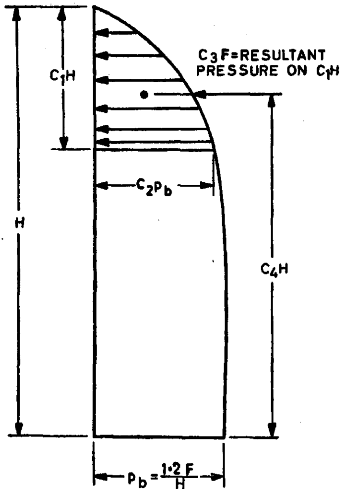
FIG. 8 DIAGRAM SHOWING PRESSURE DISTRIBUTION
