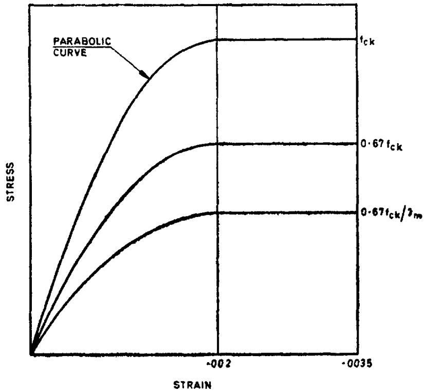
FIG. 3 STRESS STRAIN CURVE FOR CONCRETE
