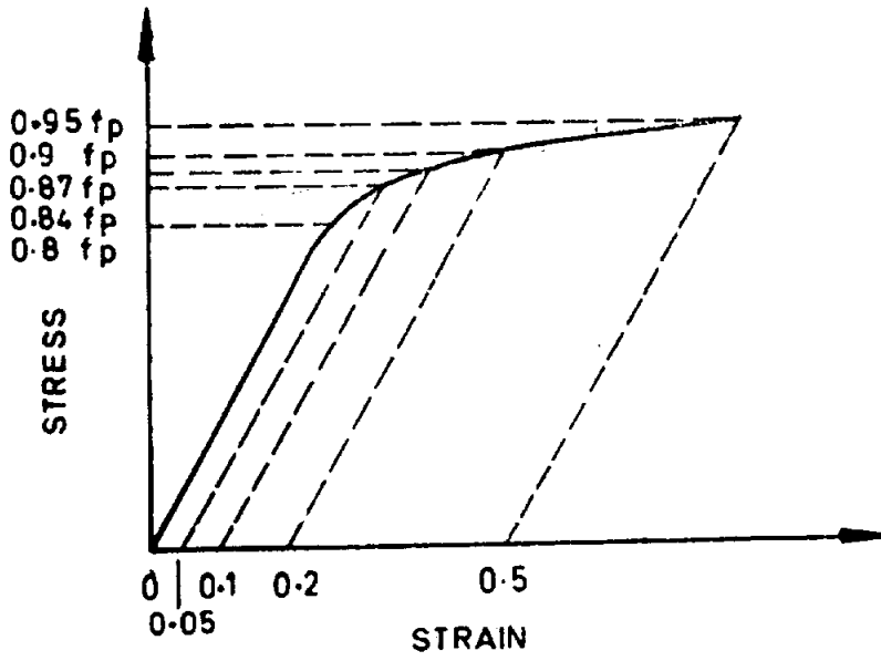
5A WIRES (STRESS RELIEVED), STRANDS AND BARS
