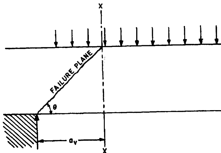
NOTE — The shear causing failure is that acting on section X-X.
