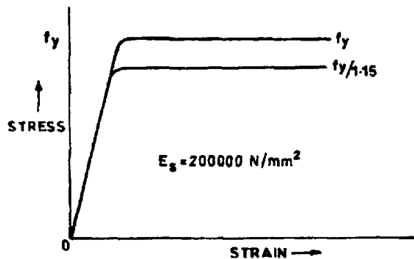
23B STEEL BAR WITH DEFINITE YIELD POINT
